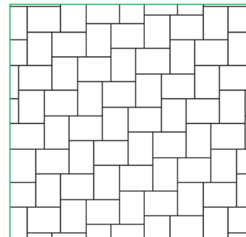
VM 26 - Liana, Rivera, Rustana Bedarf: 21x28 = 17,08 Stk/m 2
