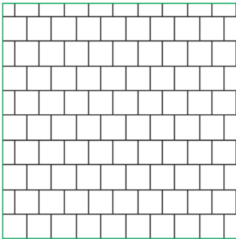
VM 07 - Liana, Rivera, Rustana Bedarf: 21x21 = 22,78 Stk/m 2
